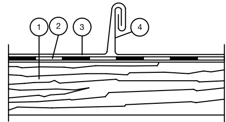
Fig. 1: Double standing seam
