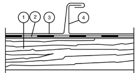
Fig. 2: Angular standing seam
